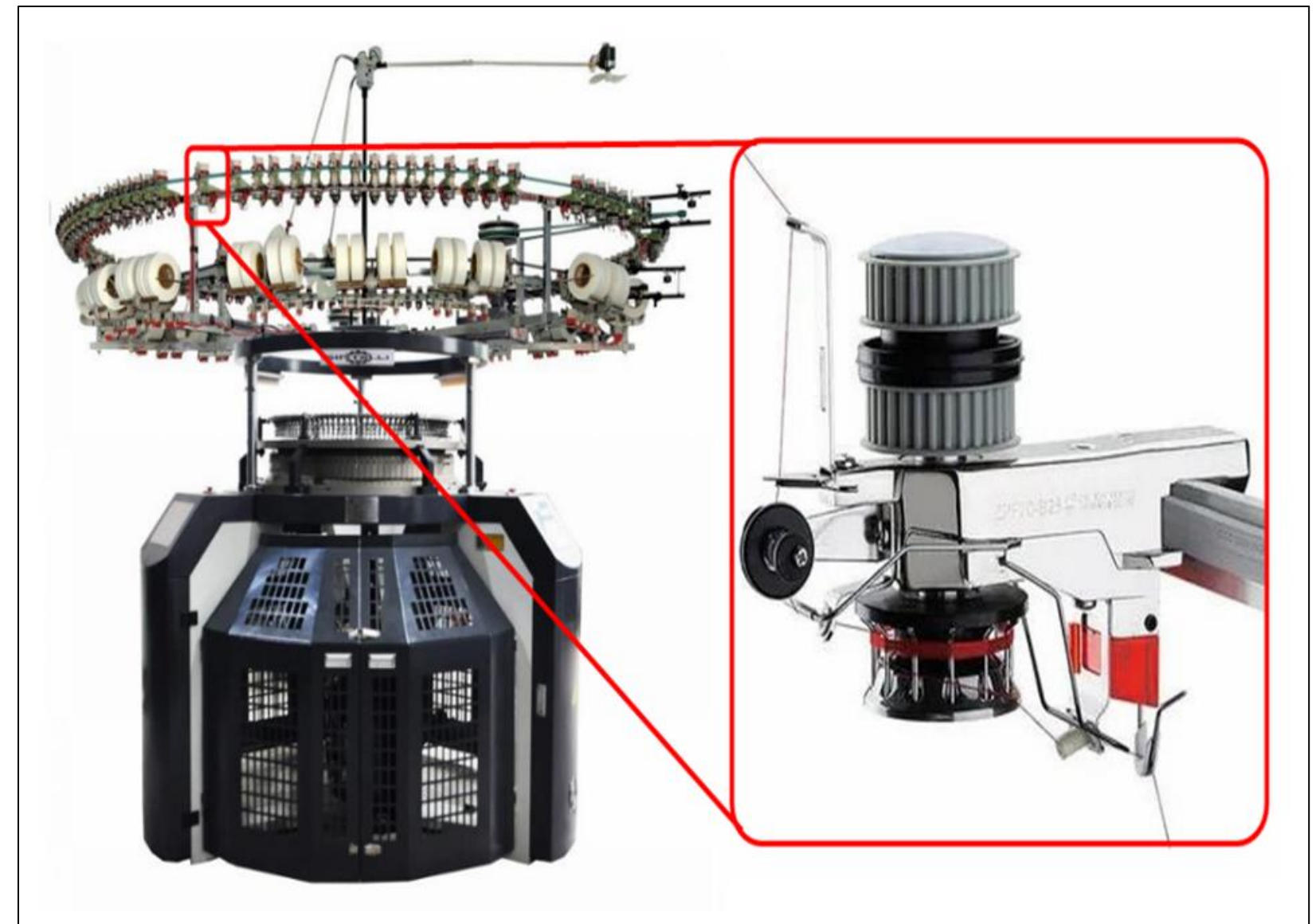
POSITIVE FEEDER
