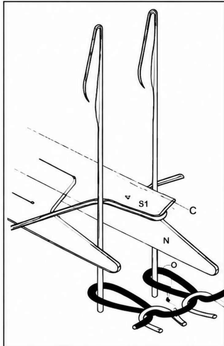
Loop forming Sinker
