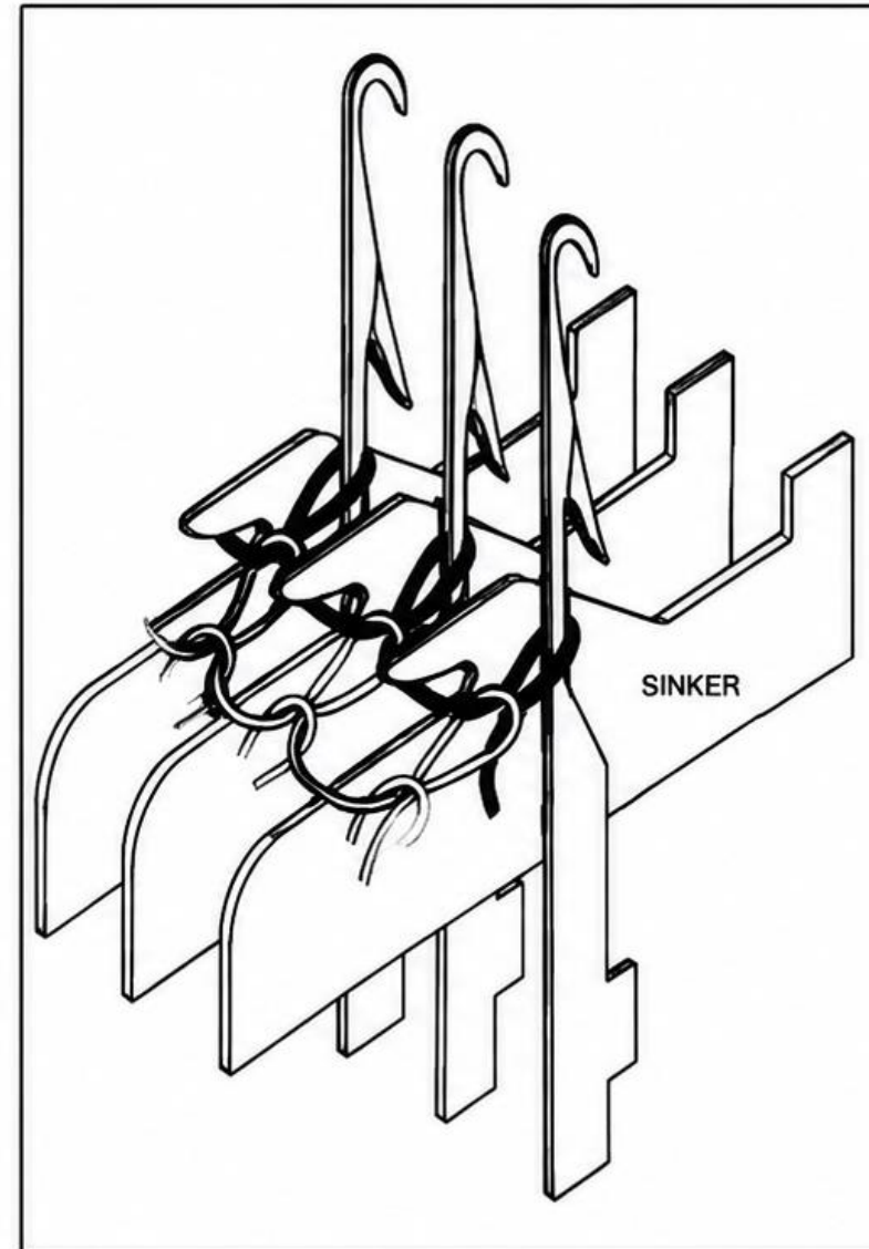
Holding – down Sinker
